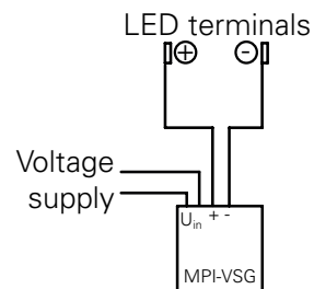
Connection diagram for 2-wire systems
