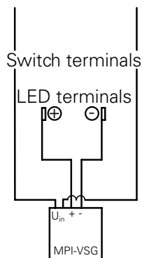
Connection diagram for 4-wire systems
